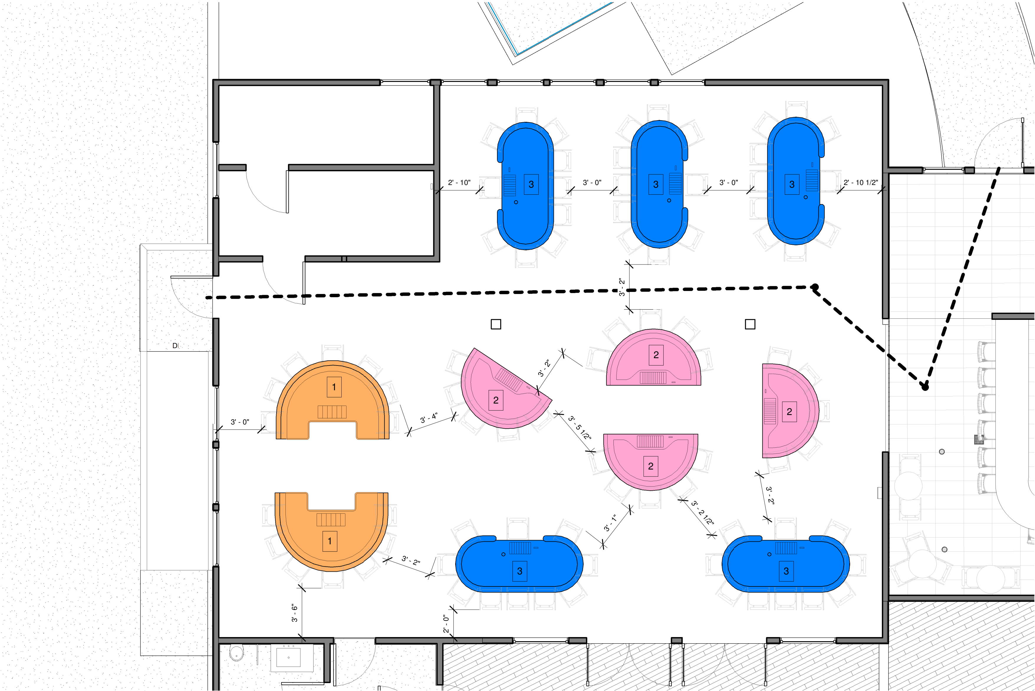
5 Level 1 - Proposed Gaming - Callout 1 1/4" = 1'-0"
